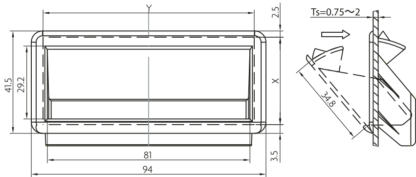
Panel cutout
